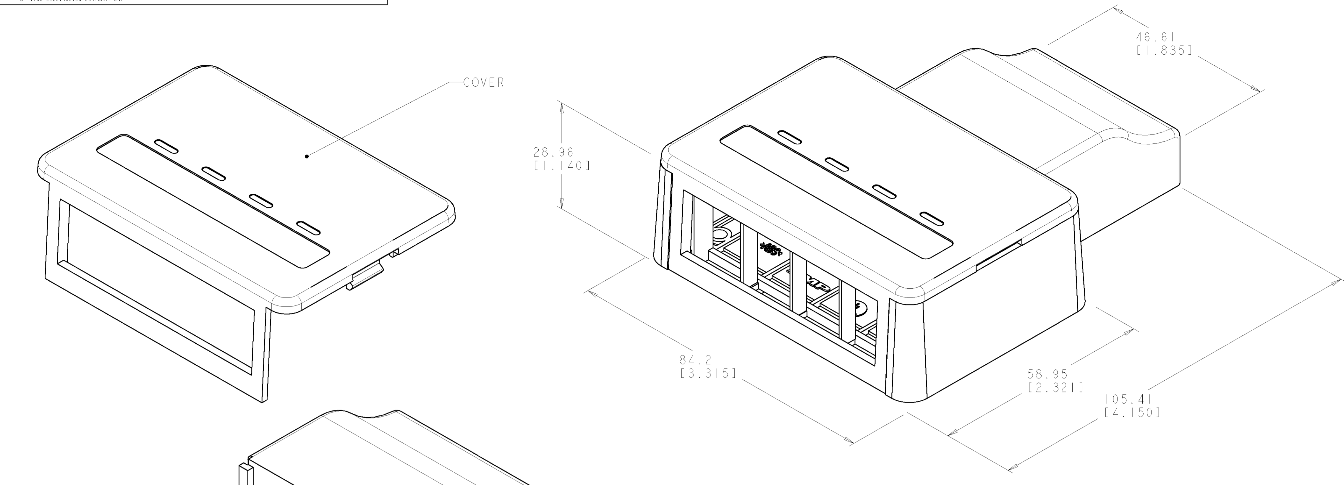
ASSEMBLED VIEW
